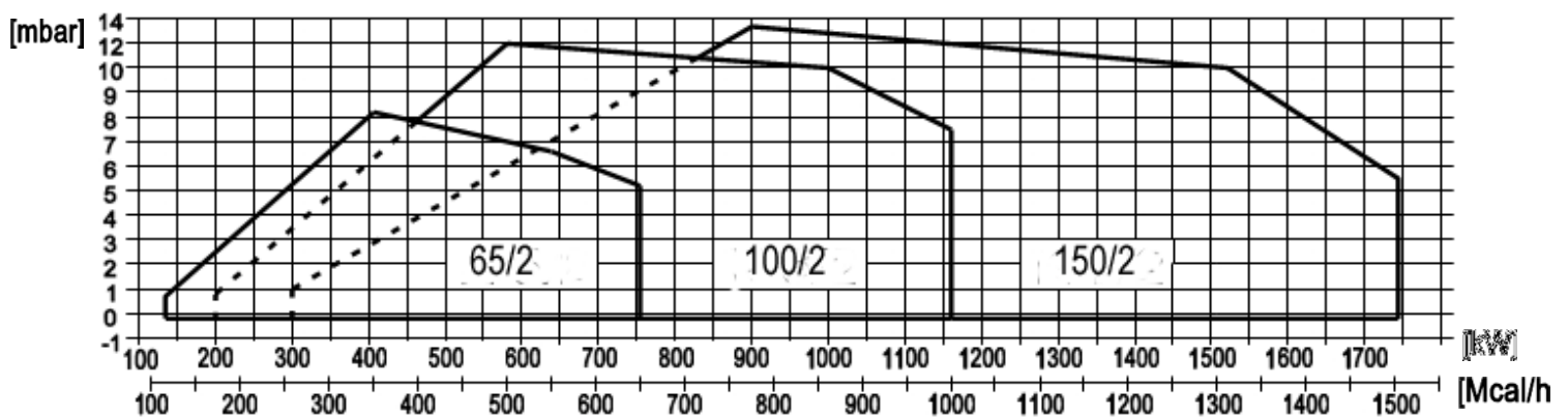
Fig. 2 X = Thermal Power Y = Pressure in combustion chamber
