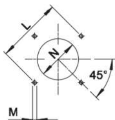
Fig. 4 Boiler plate
